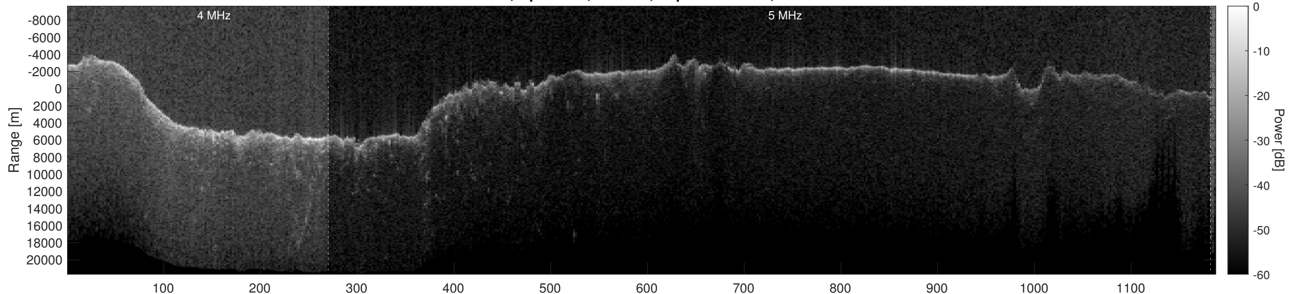
Orbit 12468, Optimized, Window, Depth-Corrected, Channel 2
