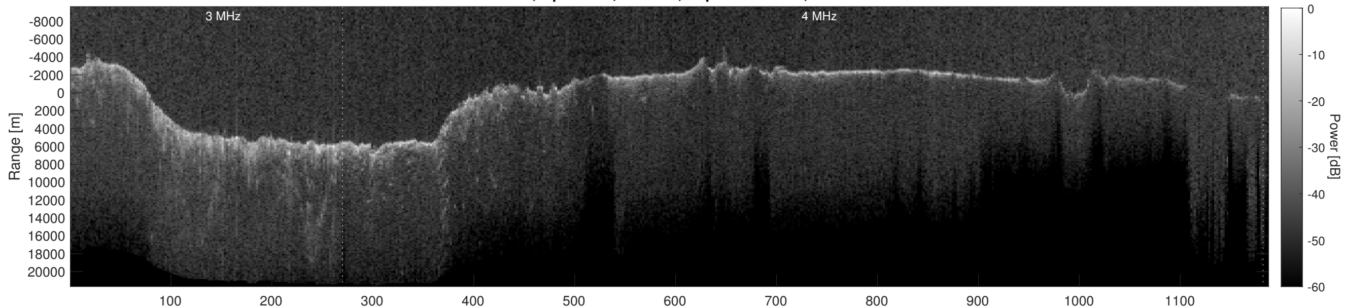
Orbit 12468, Depth-Corrected Cluttergram
