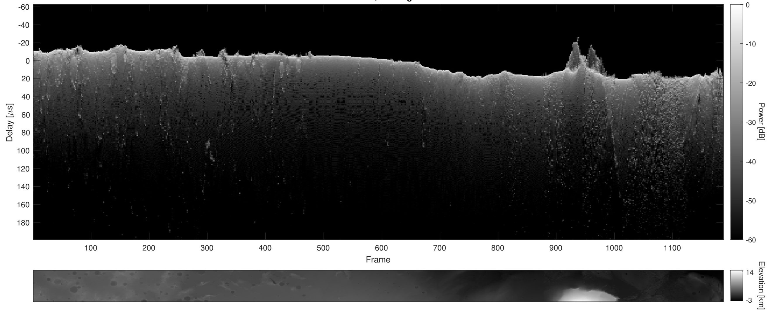
Orbit 12470, Cluttergram
