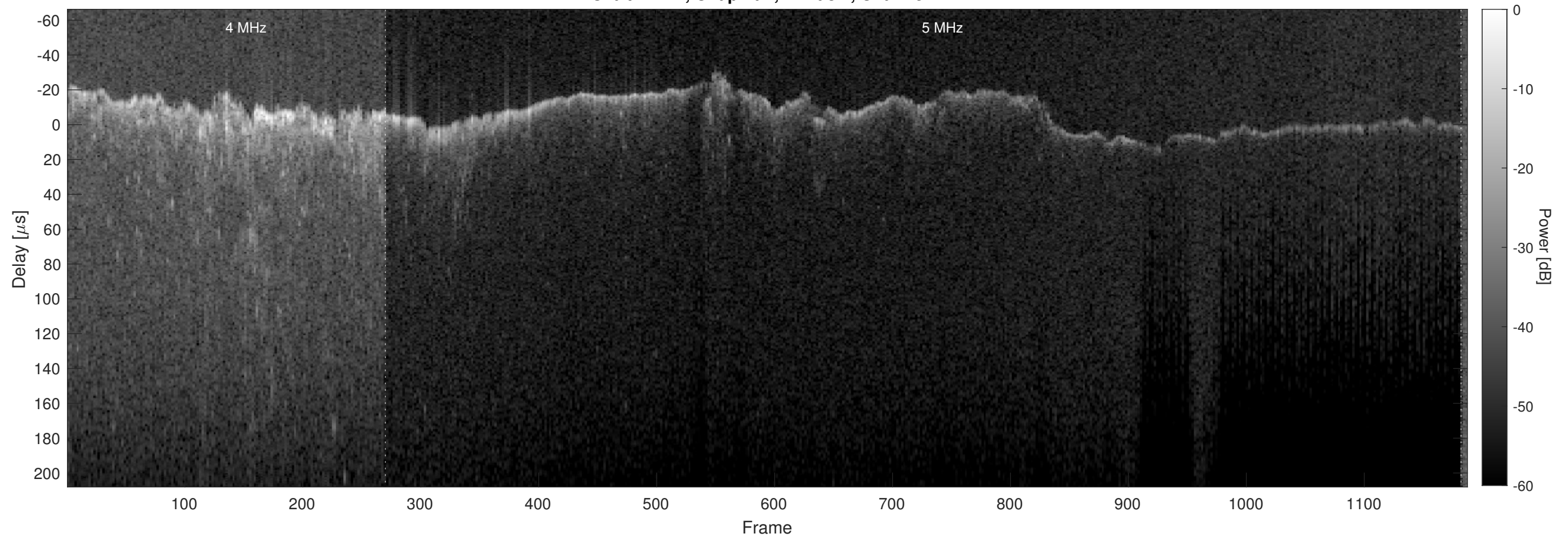
Orbit 12471, Chapman, Window, Channel 2
