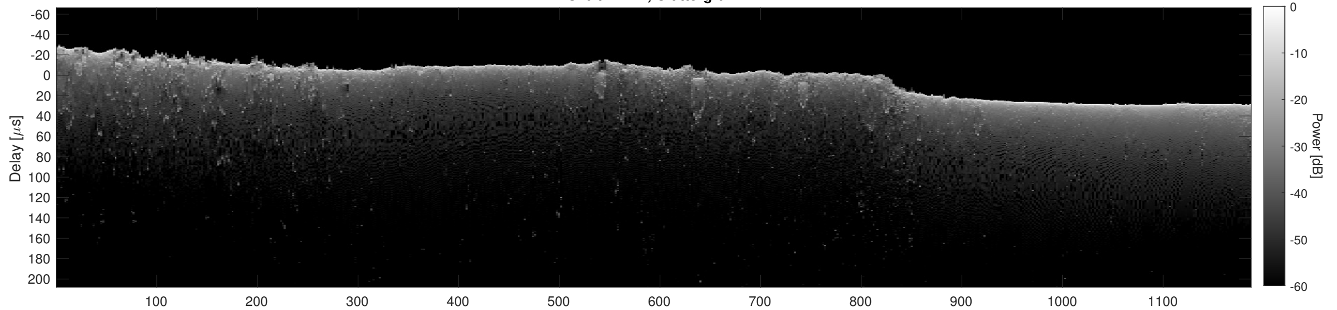
Orbit 12471, Cluttergram
