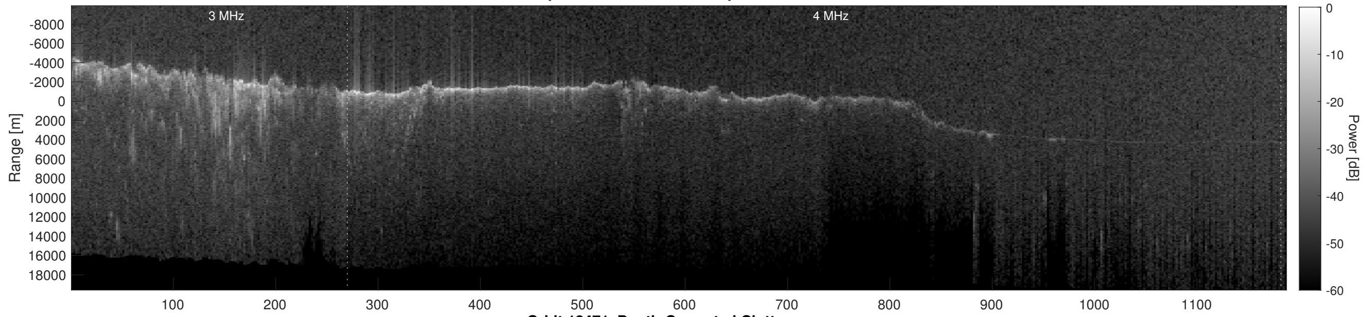
Orbit 12471, Depth-Corrected Cluttergram
