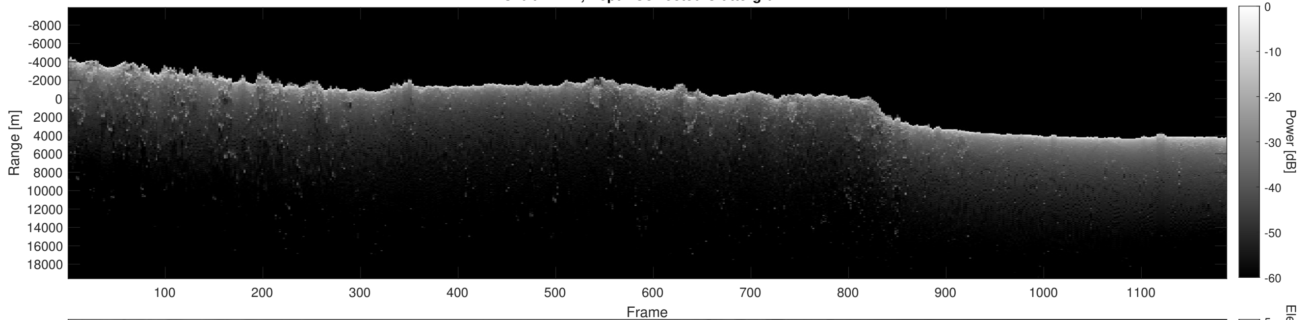
Orbit 12471, Depth-Corrected Cluttergram
