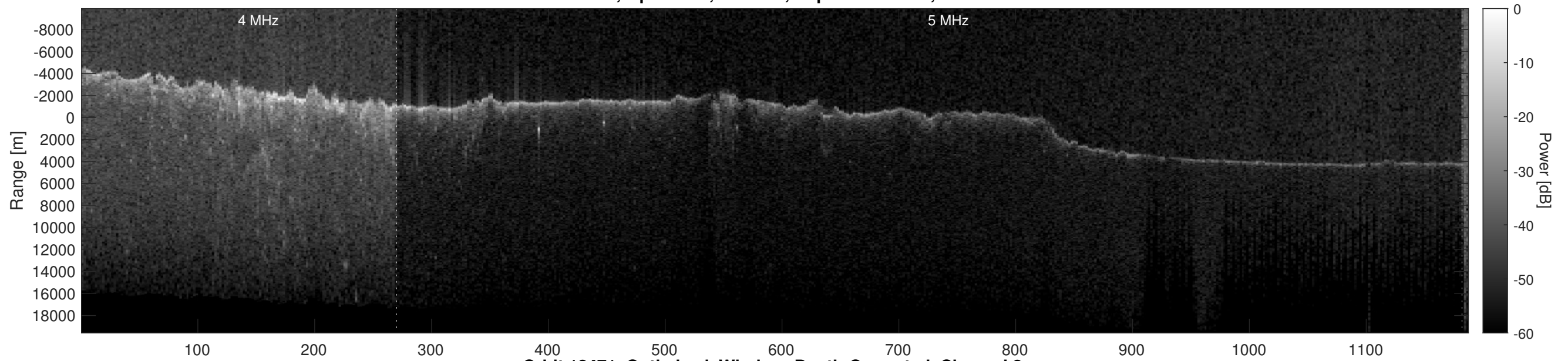
Orbit 12471, Optimized, Window, Depth-Corrected, Channel 2
