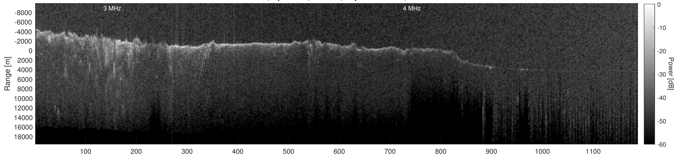
Orbit 12471, Depth-Corrected Cluttergram
