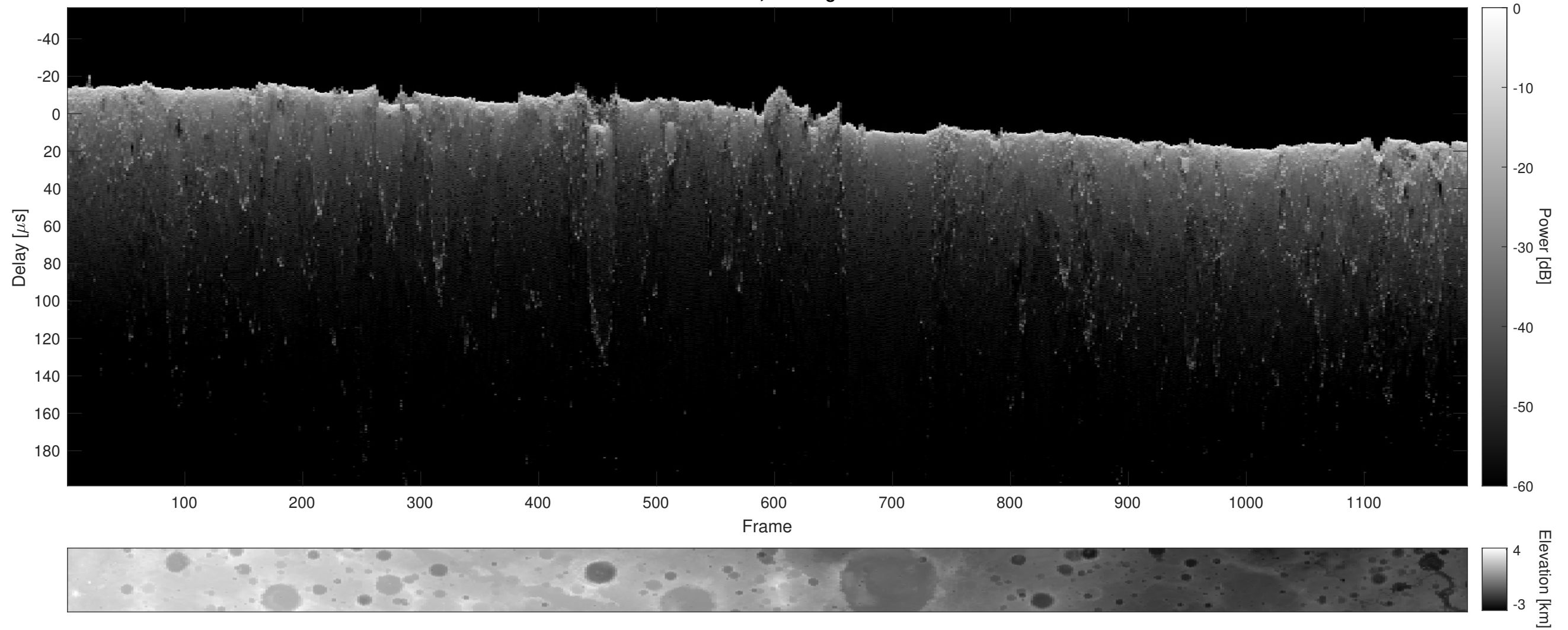
Orbit 12472, Cluttergram
