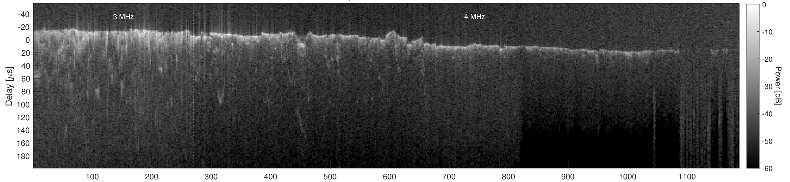
Orbit 12472, Cluttergram
