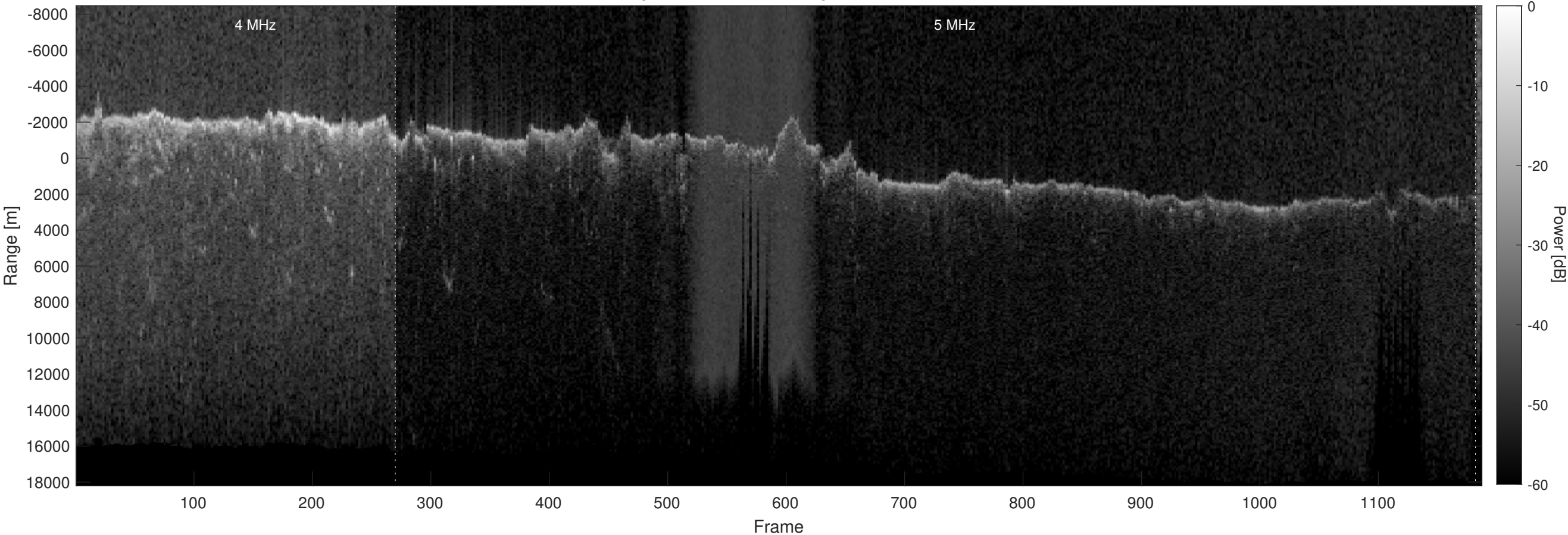
Orbit 12472, Optimized, Window, Depth-Corrected, Channel 2
