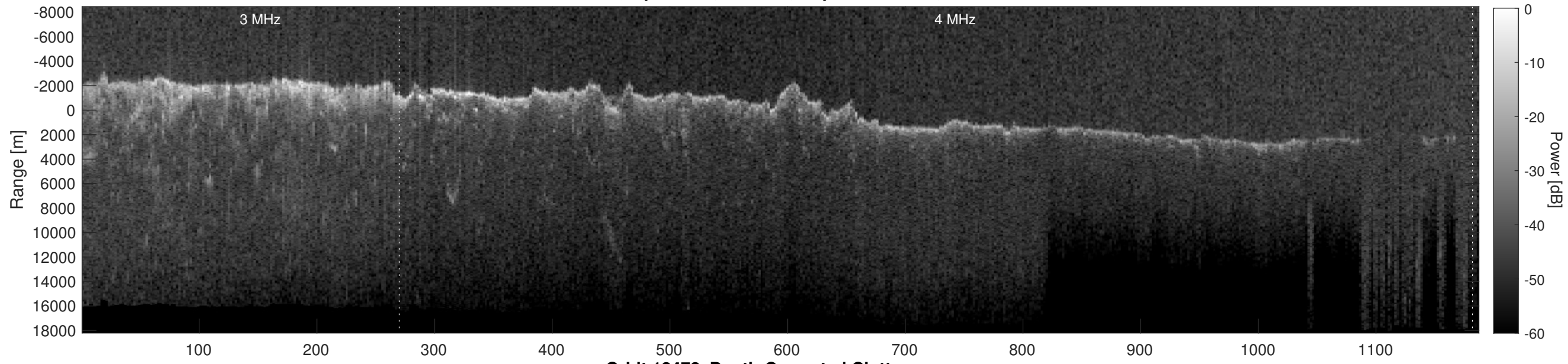
Orbit 12472, Depth-Corrected Cluttergram
