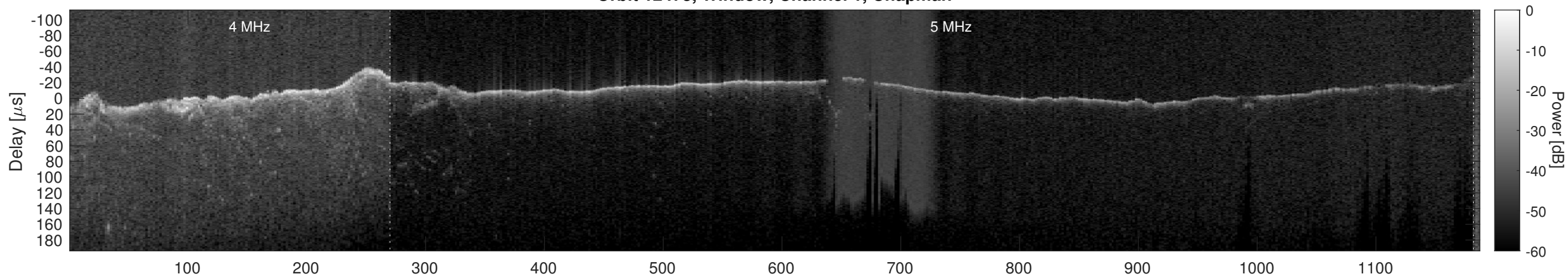
Orbit 12473, Window, Channel 1, Optimized
