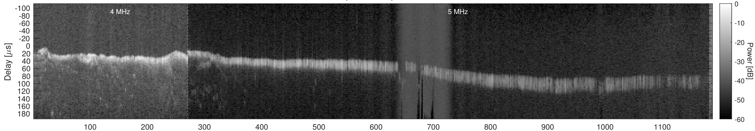
Orbit 12473, Window, Channel 1, Chapman
