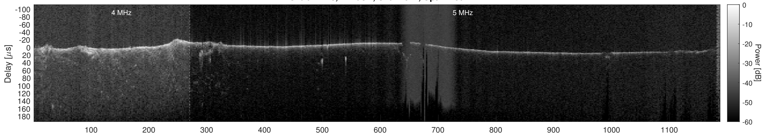
Orbit 12473, Cluttergram
