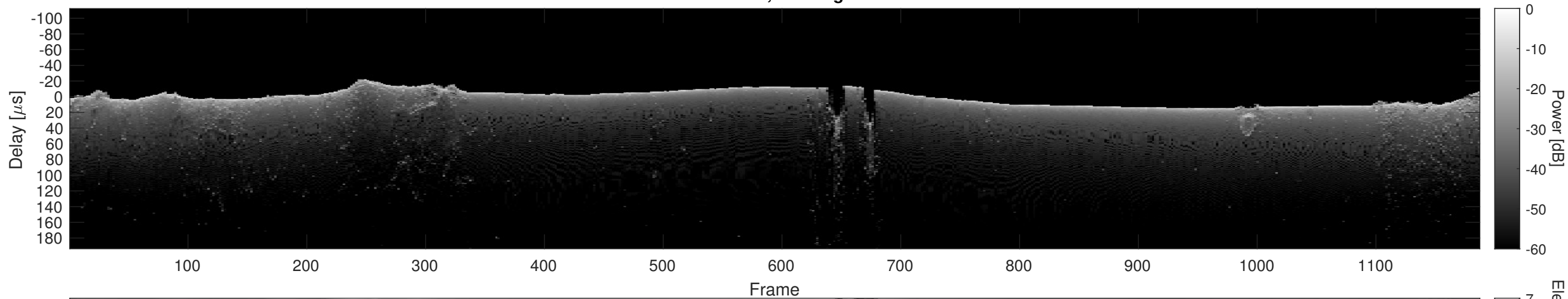
Orbit 12473, Cluttergram
