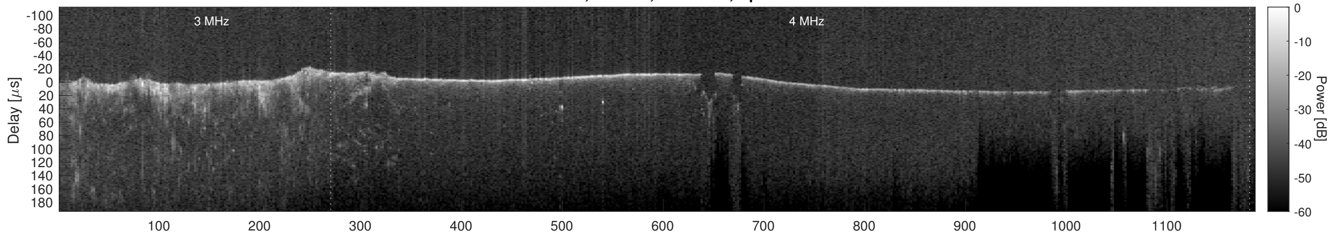
Orbit 12473, Cluttergram
