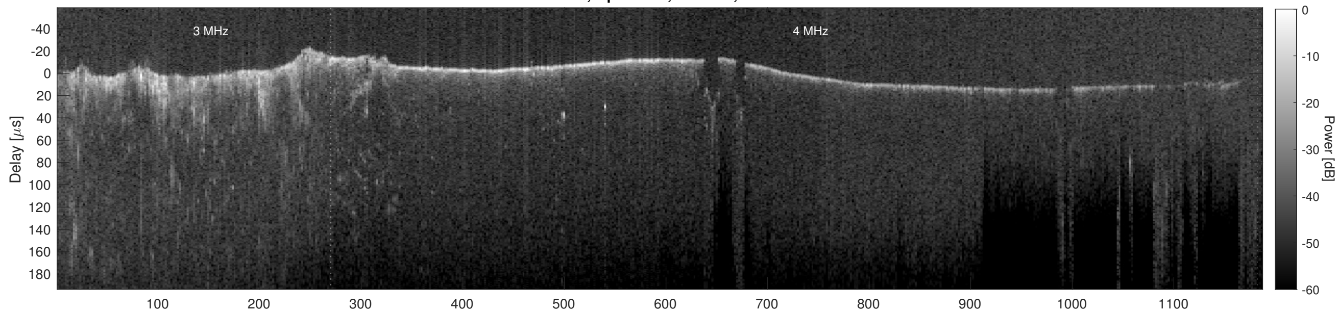
Orbit 12473, Cluttergram
