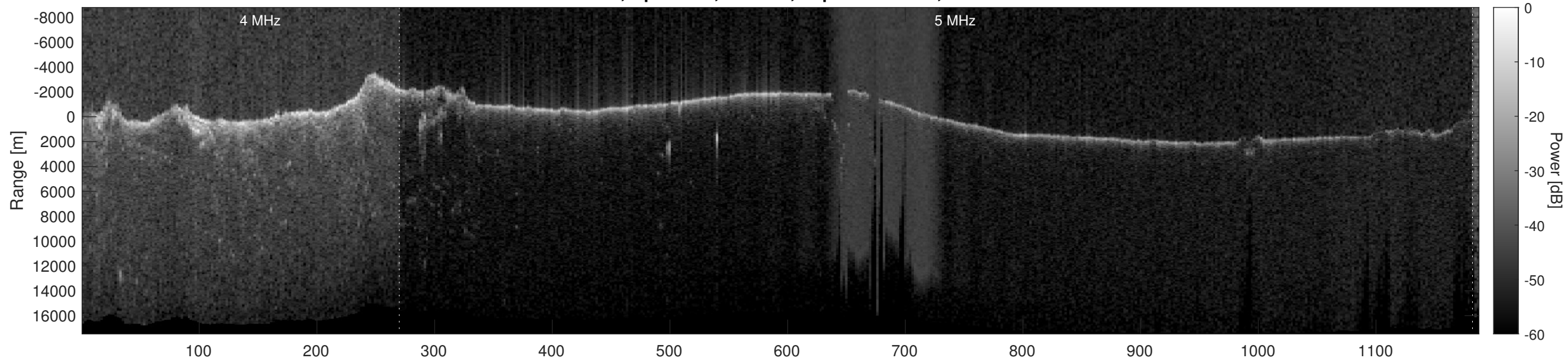
Orbit 12473, Optimized, Window, Depth-Corrected, Channel 2
