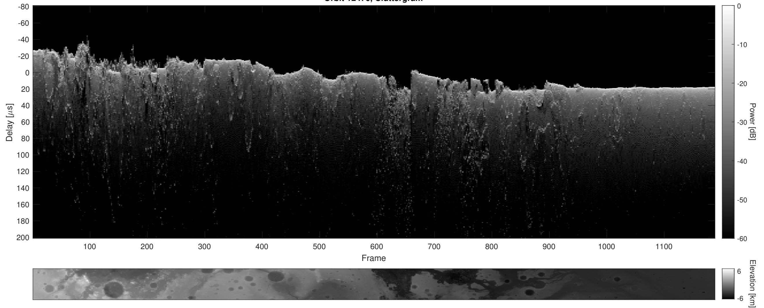
Orbit 12476, Cluttergram
