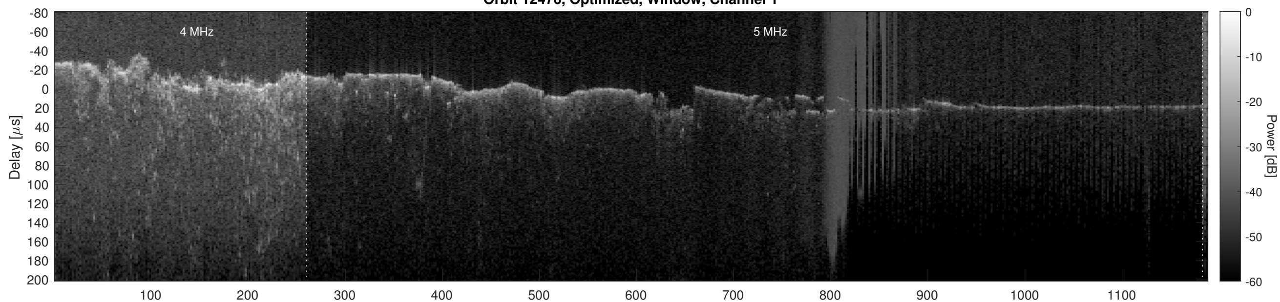
Orbit 12476, Optimized, Window, Channel 2
