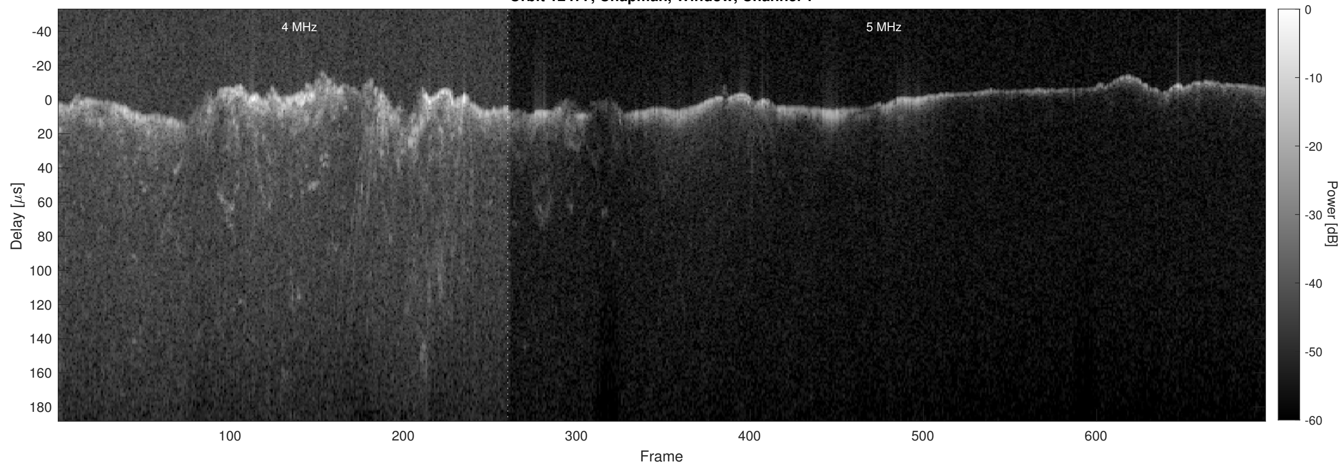
Orbit 12477, Chapman, Window, Channel 2
