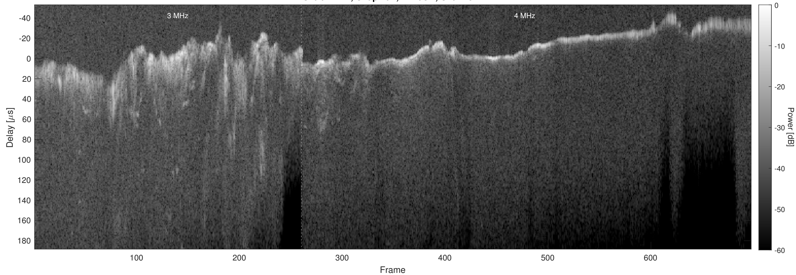
Orbit 12477, Chapman, Window, Channel 2
