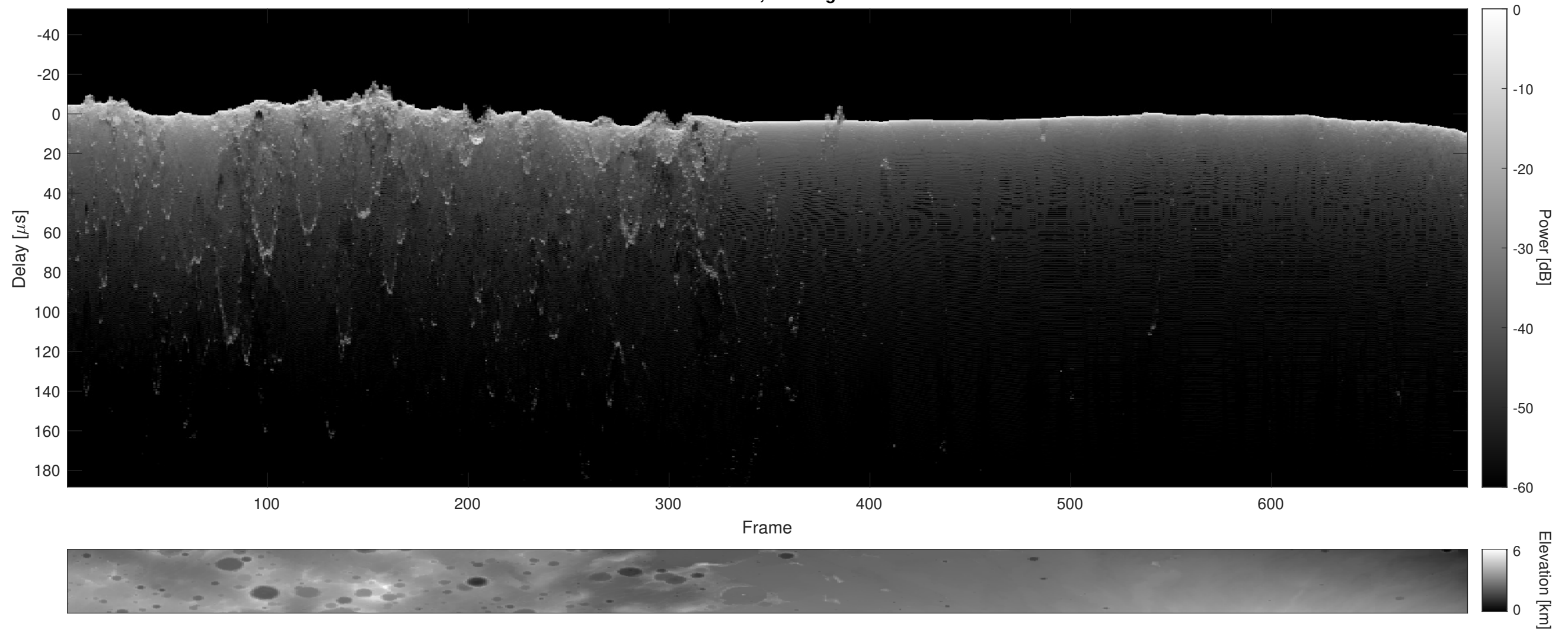
Orbit 12477, Cluttergram
