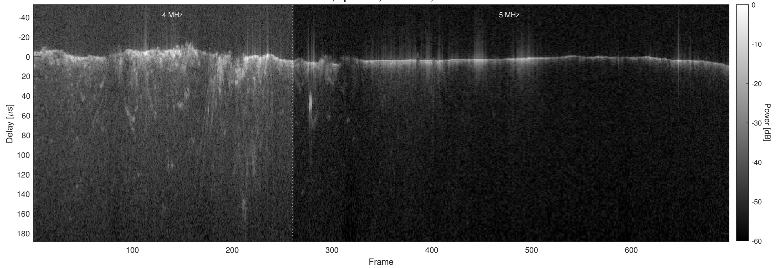
Orbit 12477, Optimized, No Window, Channel 2
