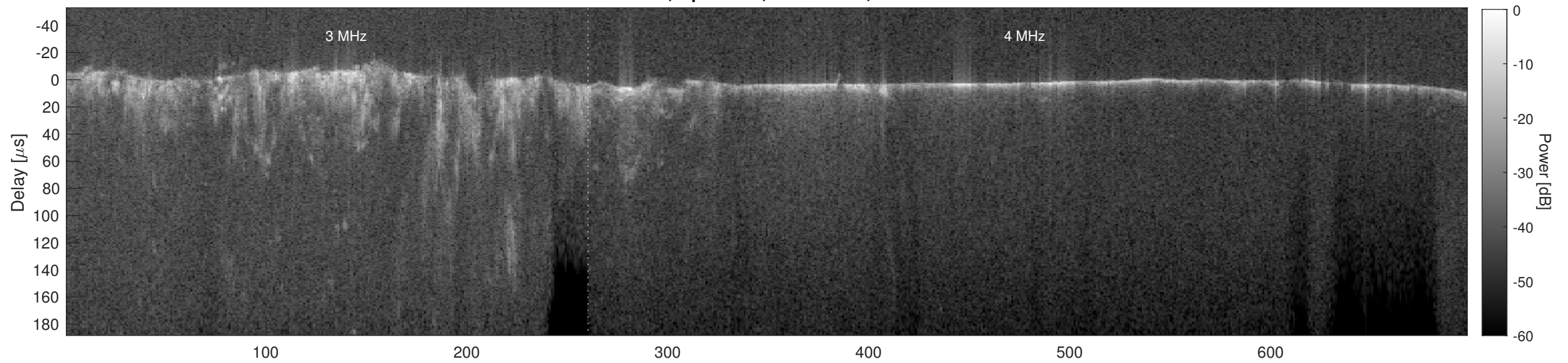
Orbit 12477, Cluttergram
