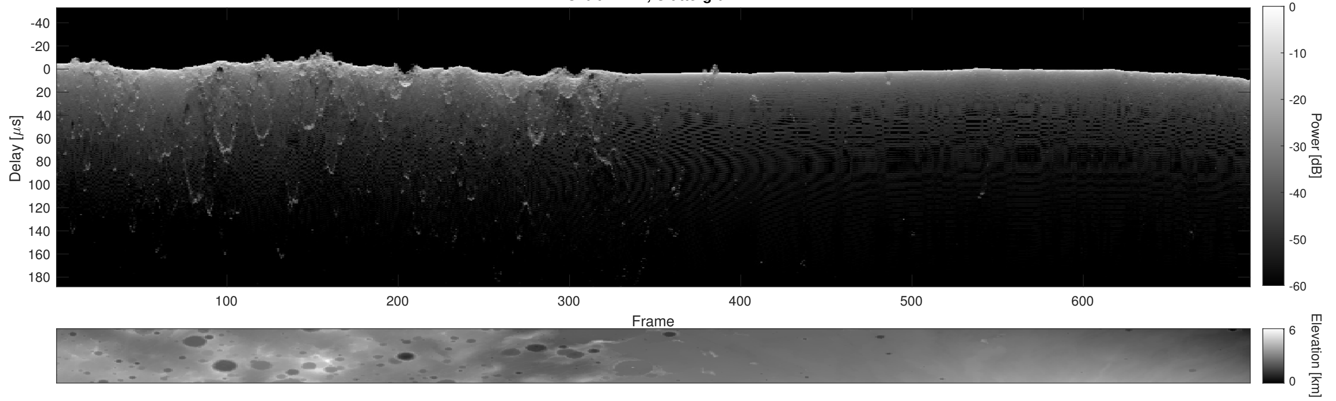
Orbit 12477, Cluttergram
