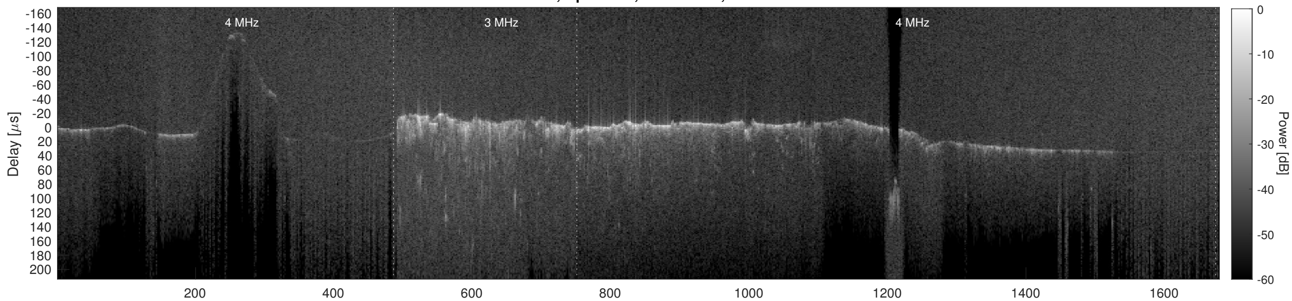
Orbit 12478, Cluttergram
