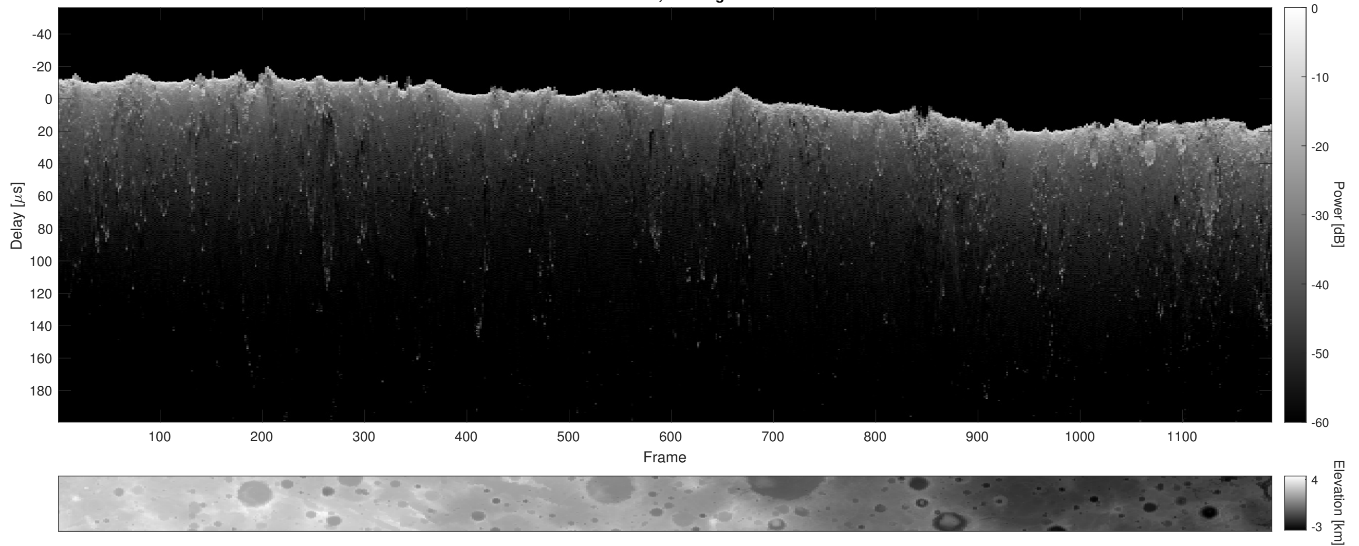
Orbit 12479, Cluttergram
