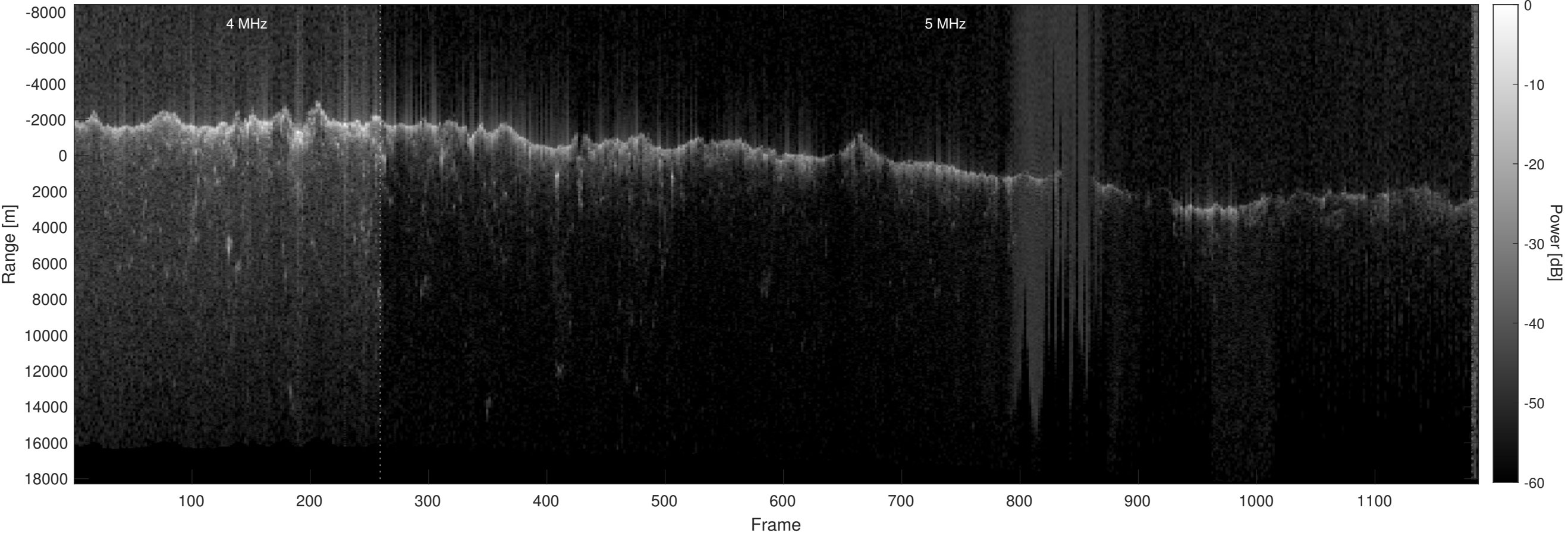
Orbit 12479, Optimized, No Window, Depth-Corrected, Channel 2
