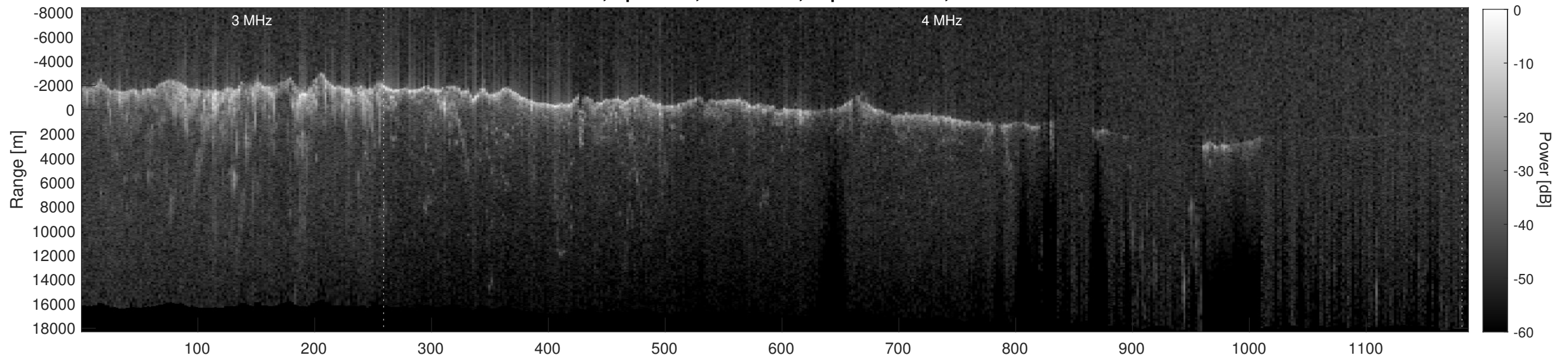
Orbit 12479, Depth-Corrected Cluttergram
