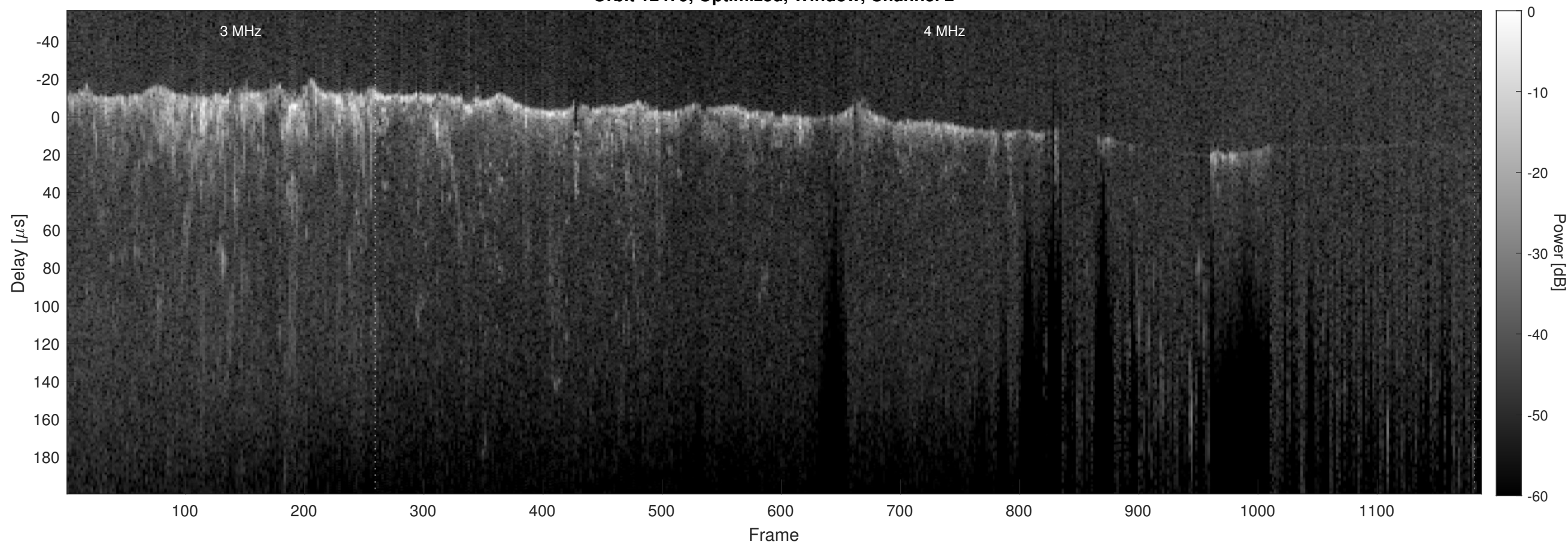
Orbit 12479, Optimized, Window, Channel 2
