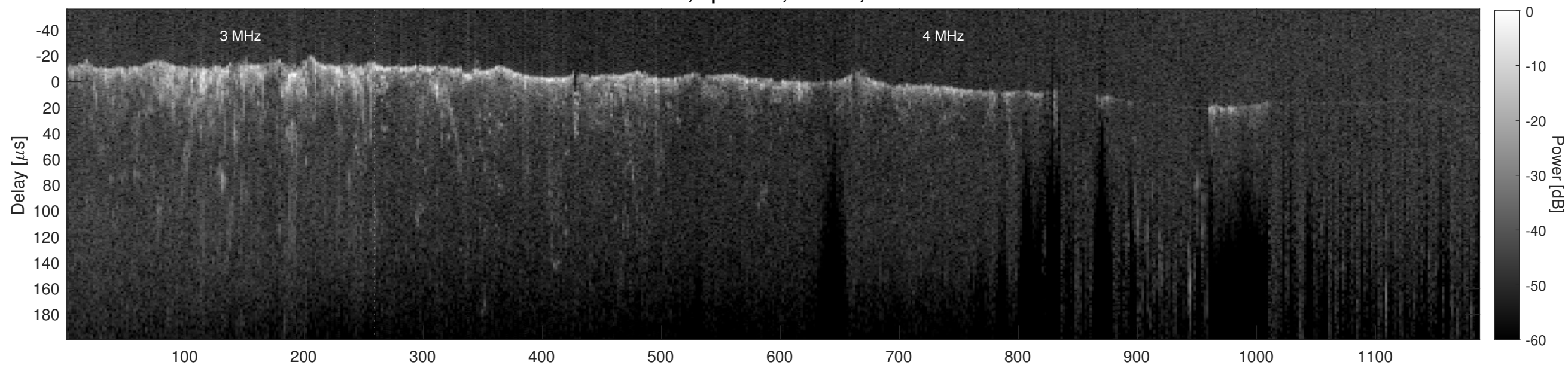
Orbit 12479, Cluttergram
