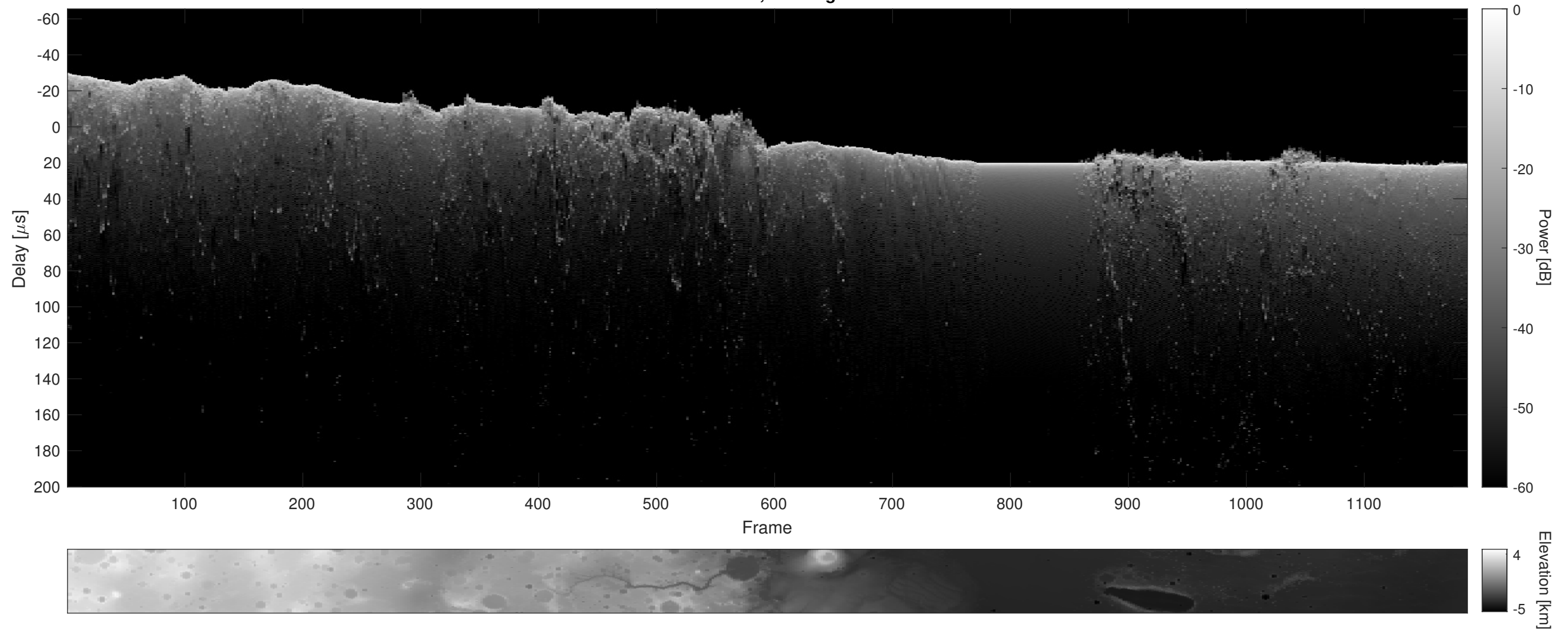
Orbit 12481, Cluttergram
