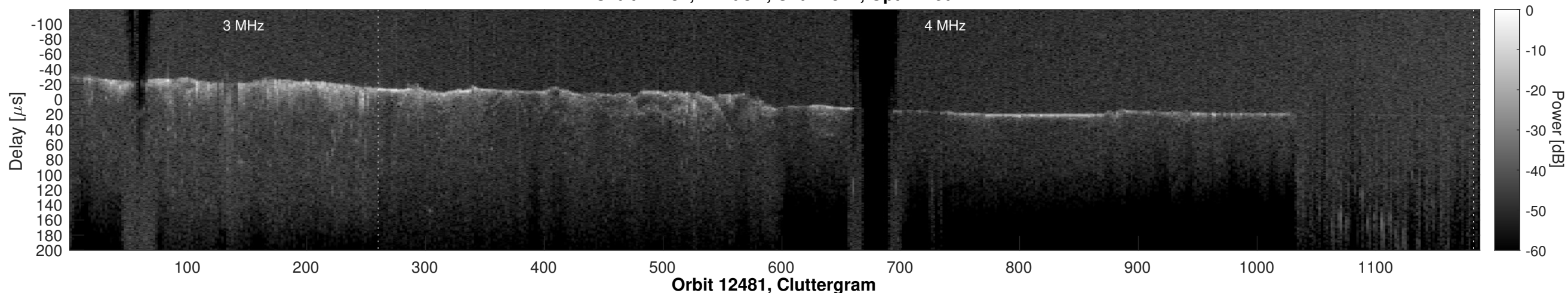
Orbit 12481, Window, Channel 2, Optimized
