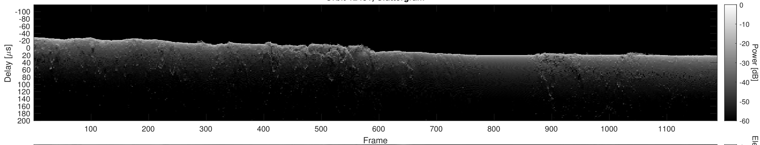
Orbit 12481, Cluttergram
