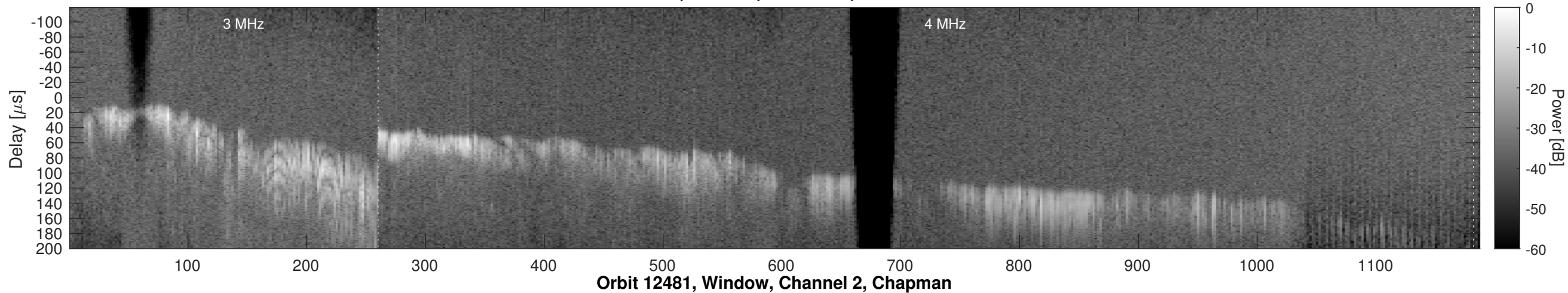
Orbit 12481, Window, Channel 2, Uncorrected
