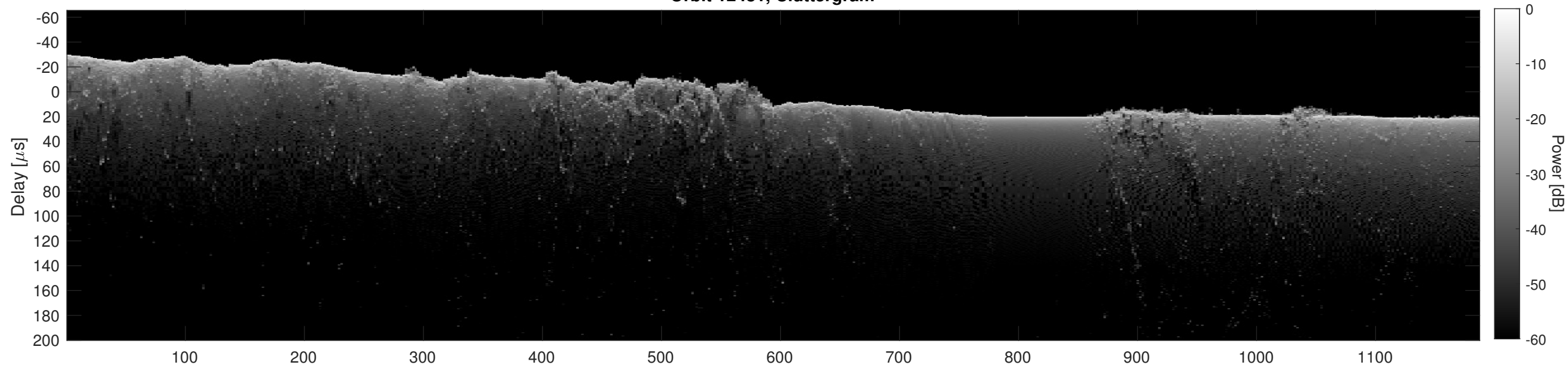
Orbit 12481, Cluttergram
