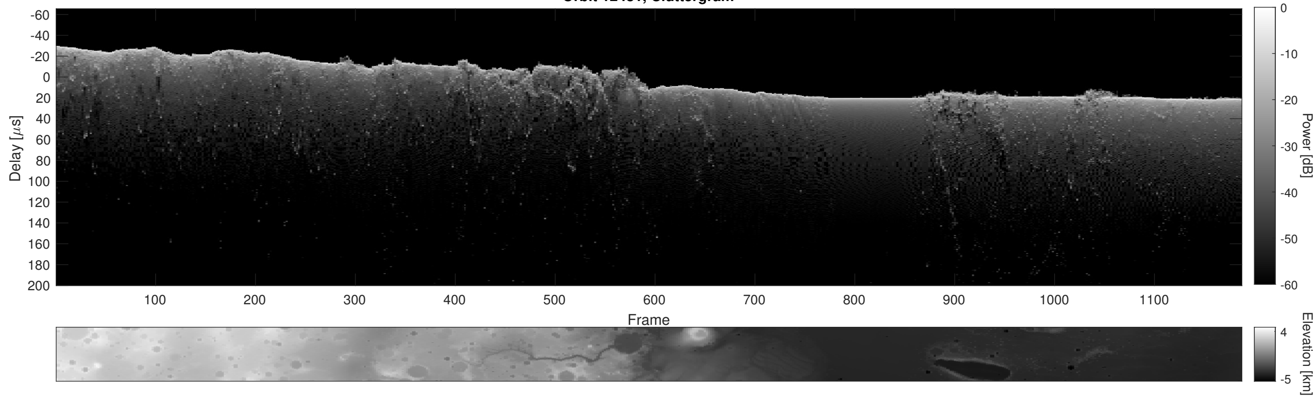
Orbit 12481, Cluttergram
