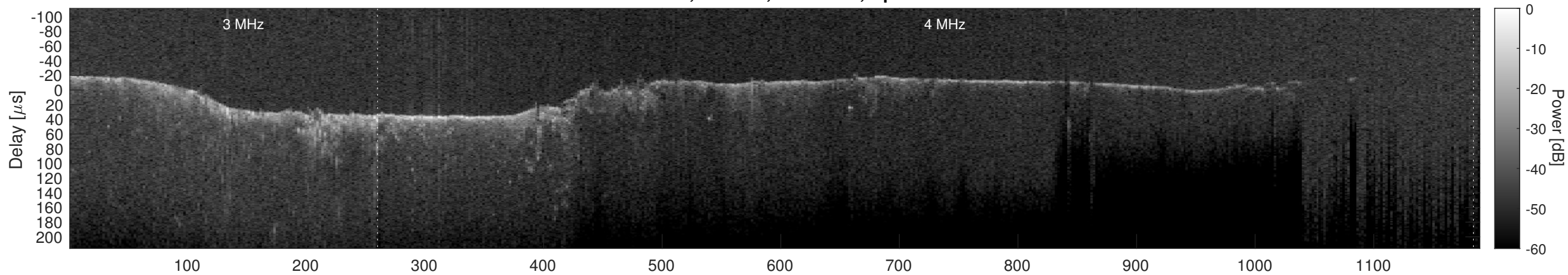
Orbit 12482, Cluttergram
