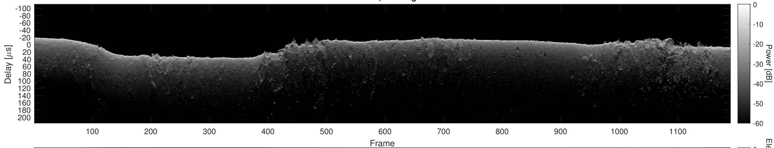
Orbit 12482, Cluttergram
