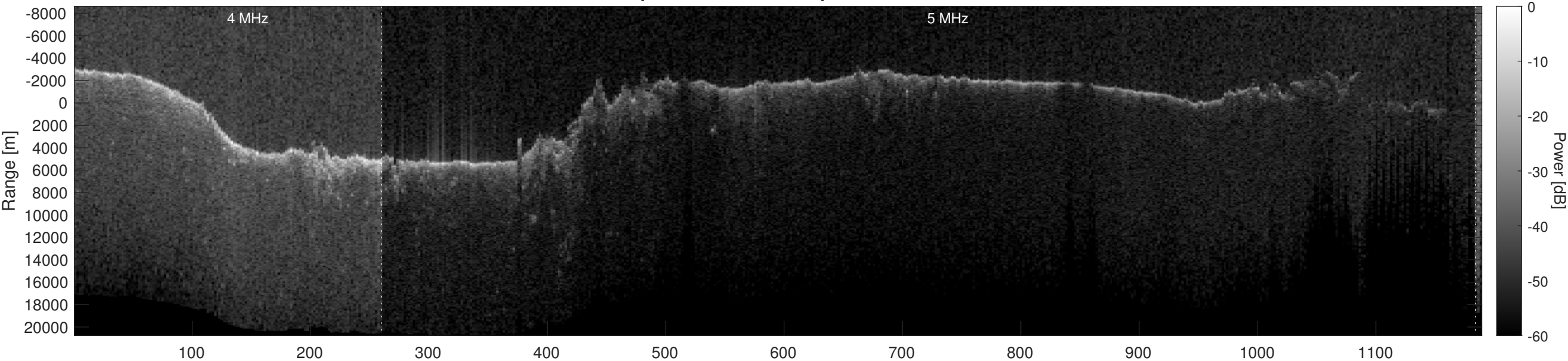
Orbit 12482, Optimized, Window, Depth-Corrected, Channel 2
