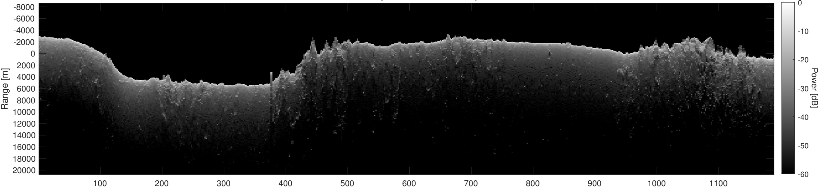
Orbit 12482, Depth-Corrected Cluttergram
