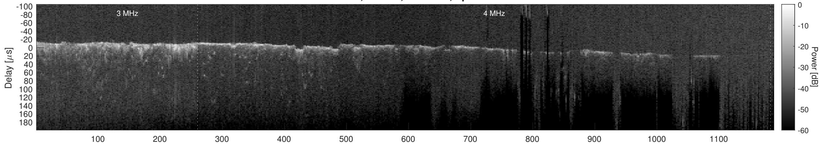
Orbit 12486, Cluttergram
