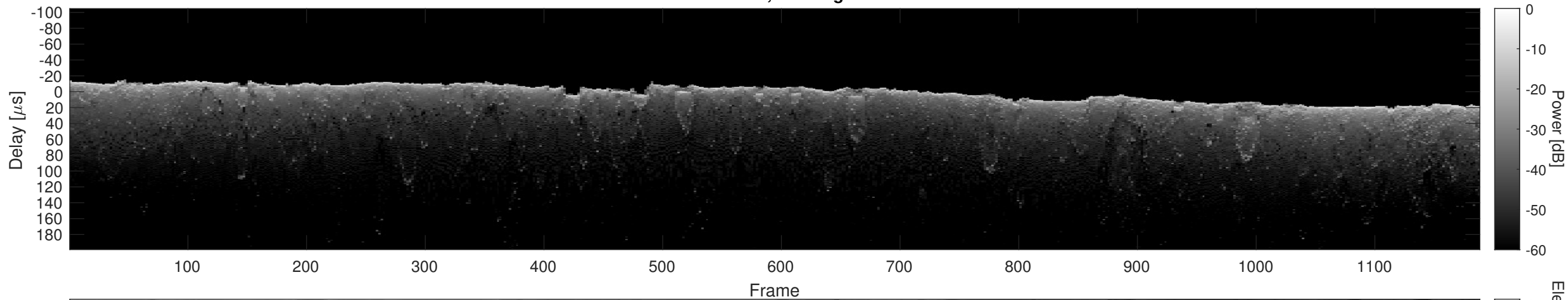
Orbit 12486, Cluttergram
