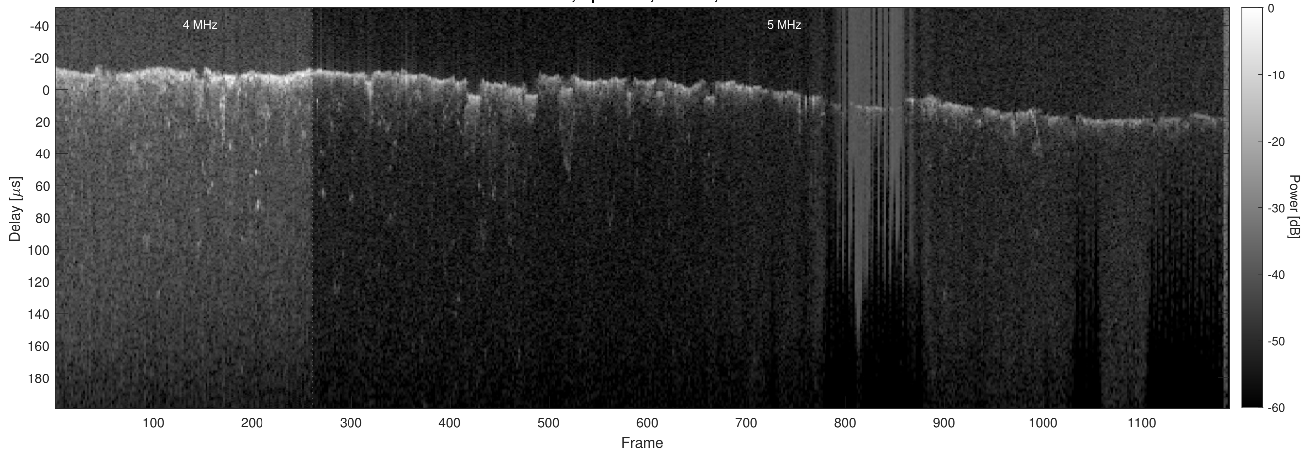
Orbit 12486, Optimized, Window, Channel 2
