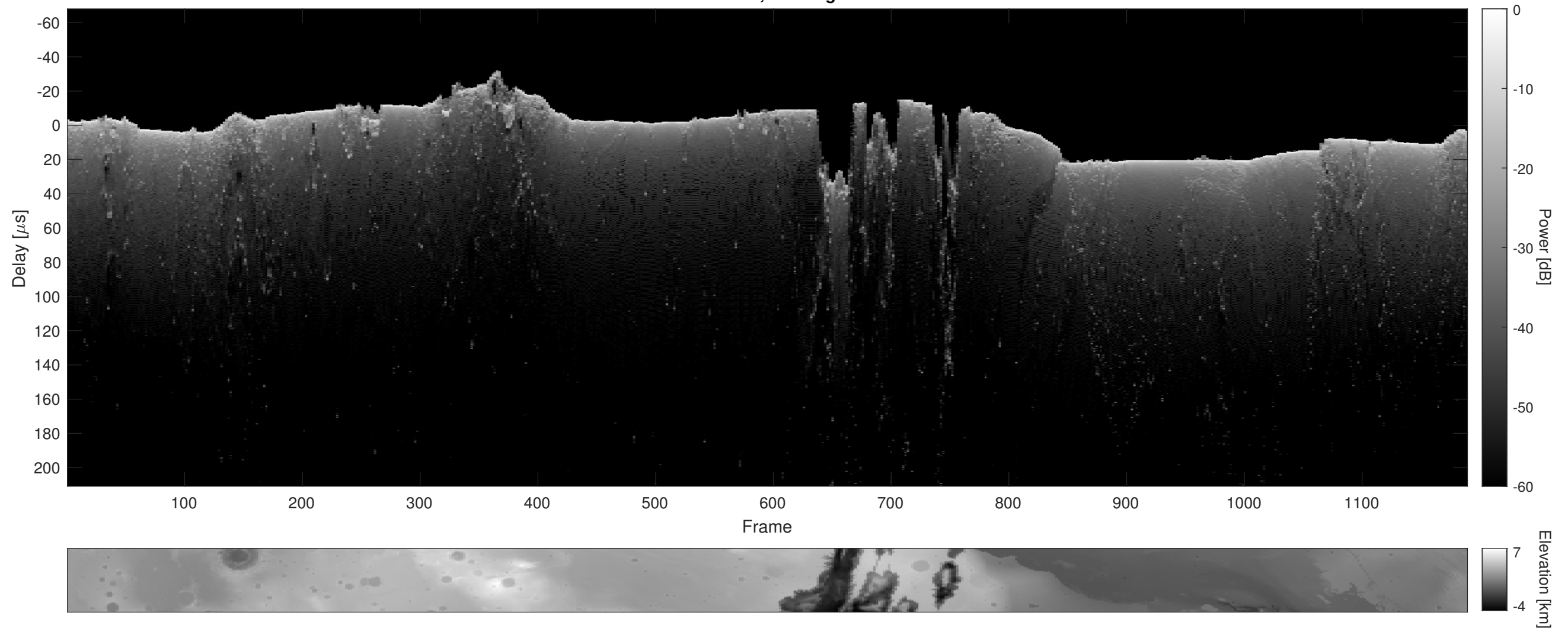
Orbit 12487, Cluttergram
