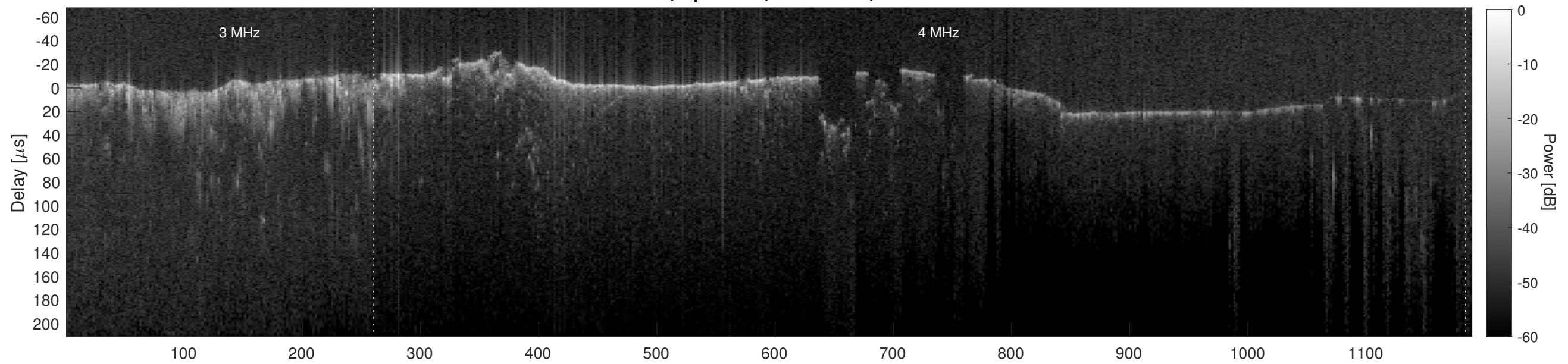
Orbit 12487, Cluttergram
