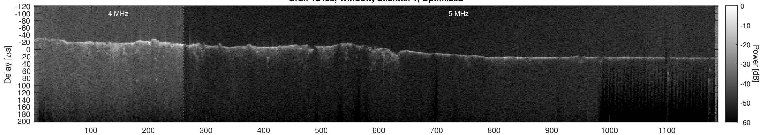
Orbit 12488, Cluttergram
