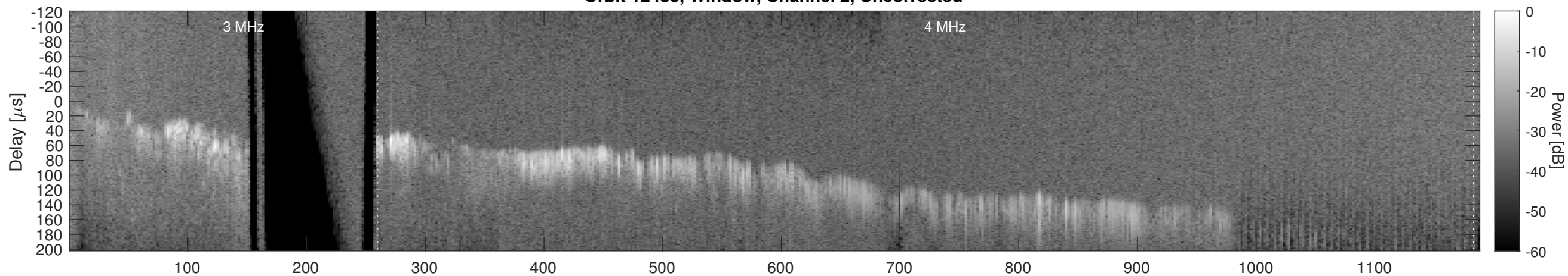
Orbit 12488, Window, Channel 2, Chapman
