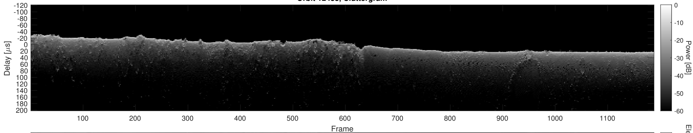
Orbit 12488, Cluttergram
