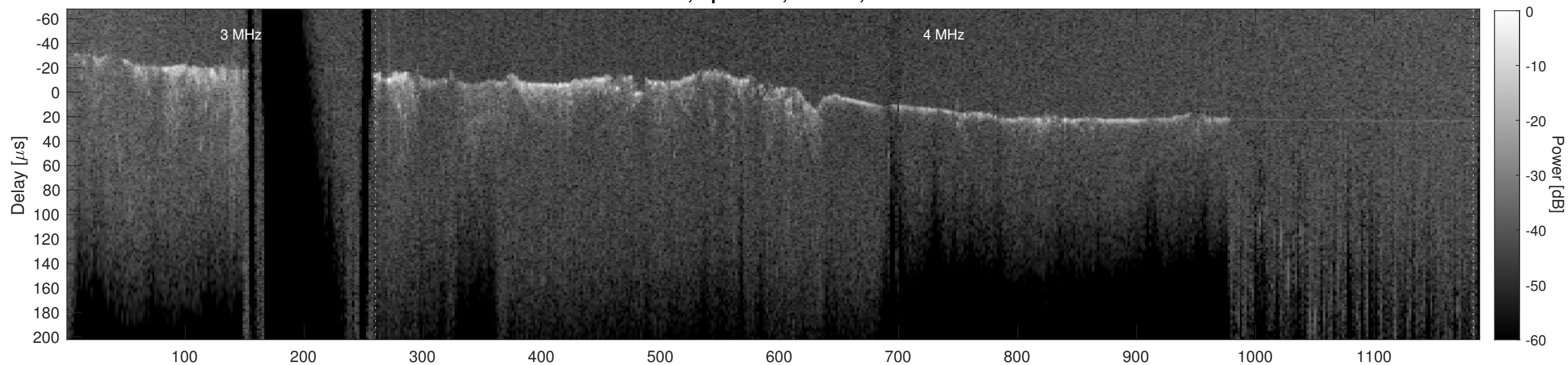
Orbit 12488, Cluttergram
