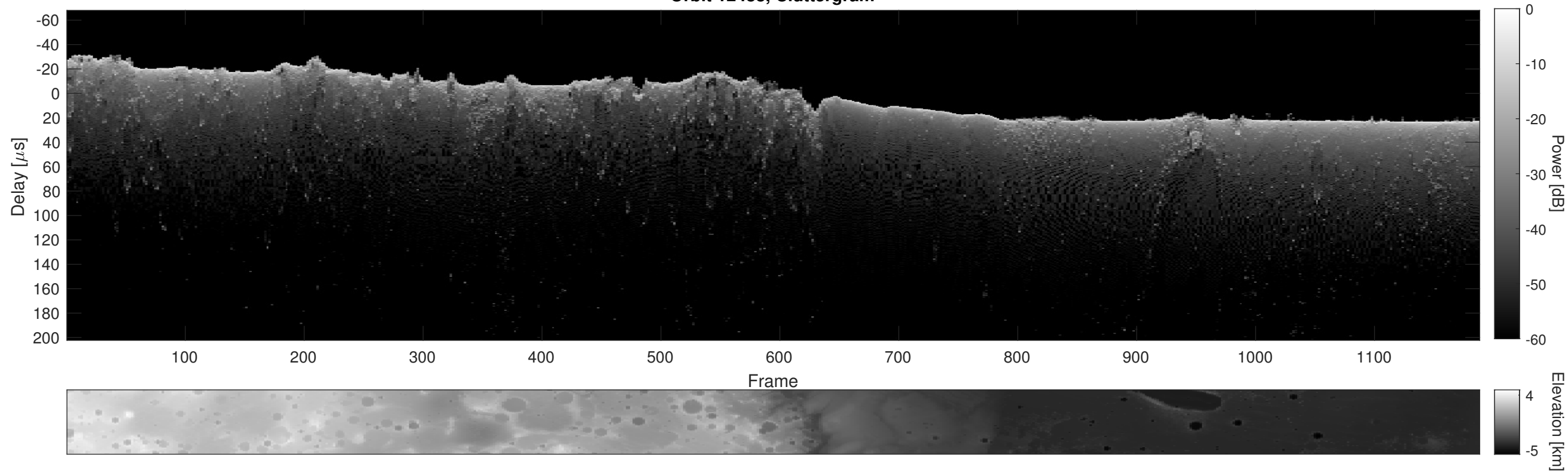
Orbit 12488, Cluttergram
