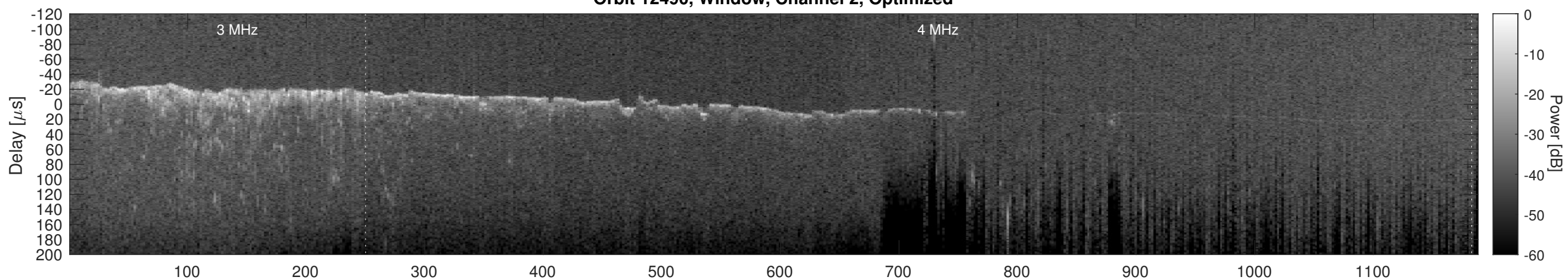
Orbit 12490, Cluttergram
