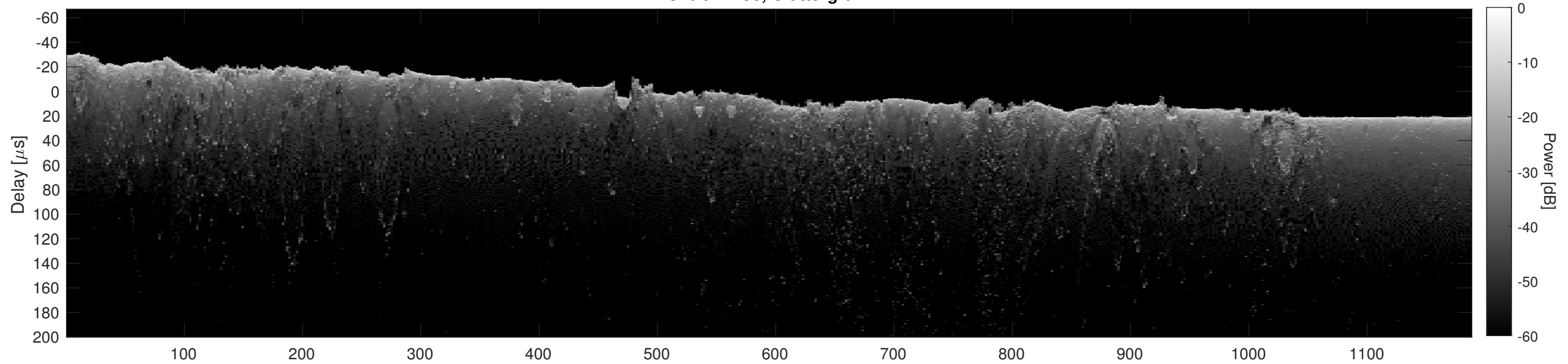
Orbit 12490, Cluttergram
