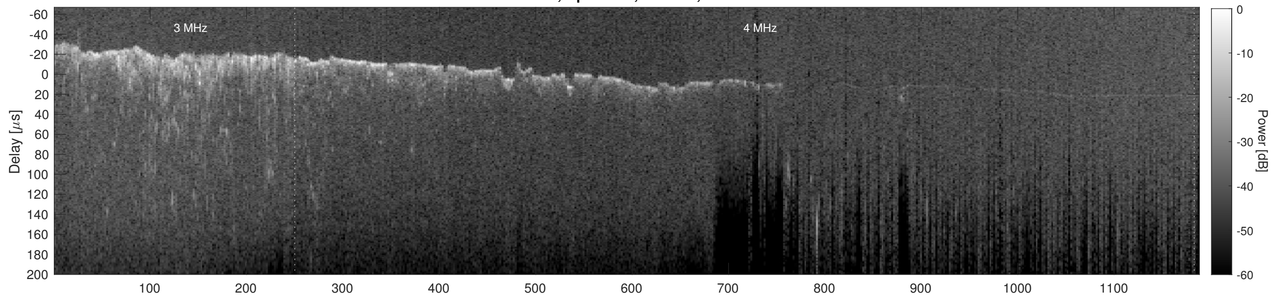
Orbit 12490, Cluttergram
