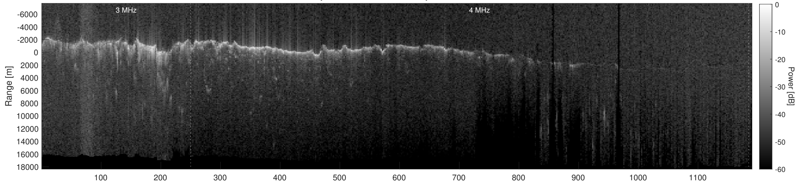
Orbit 12493, Depth-Corrected Cluttergram
