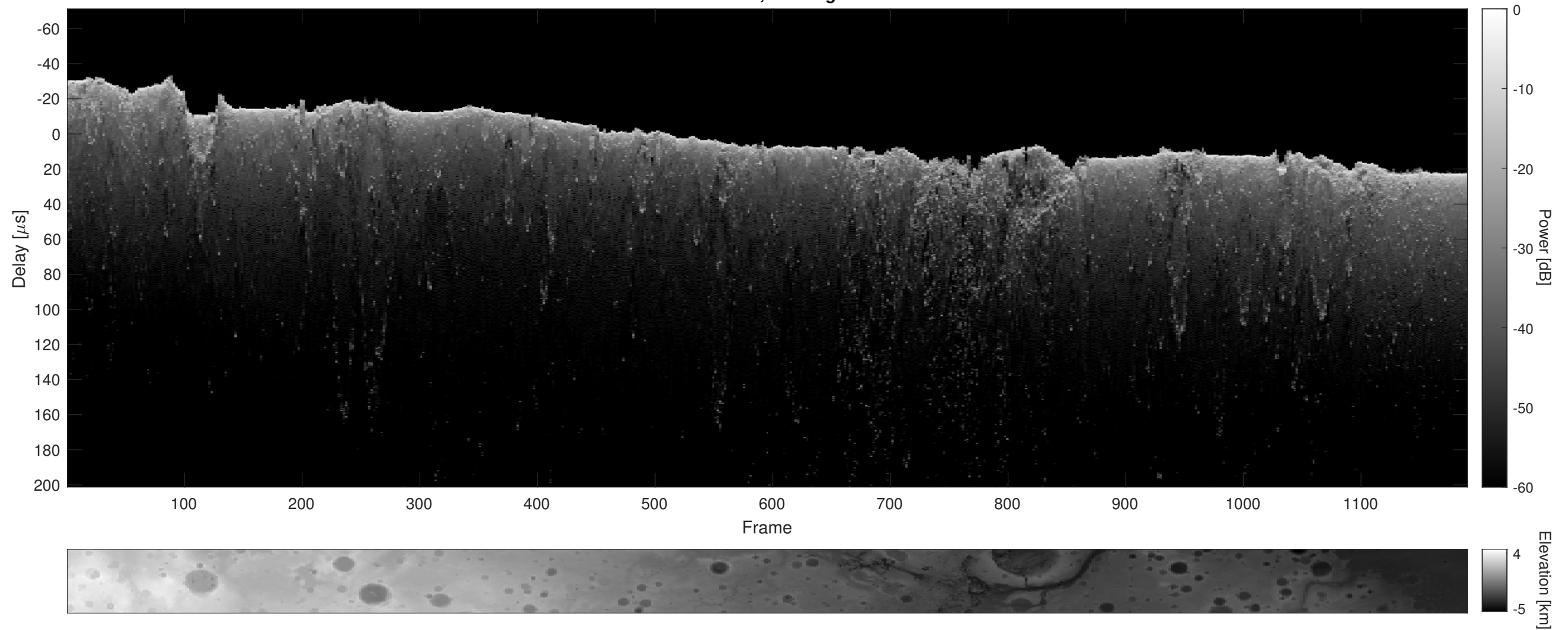
Orbit 12497, Cluttergram
