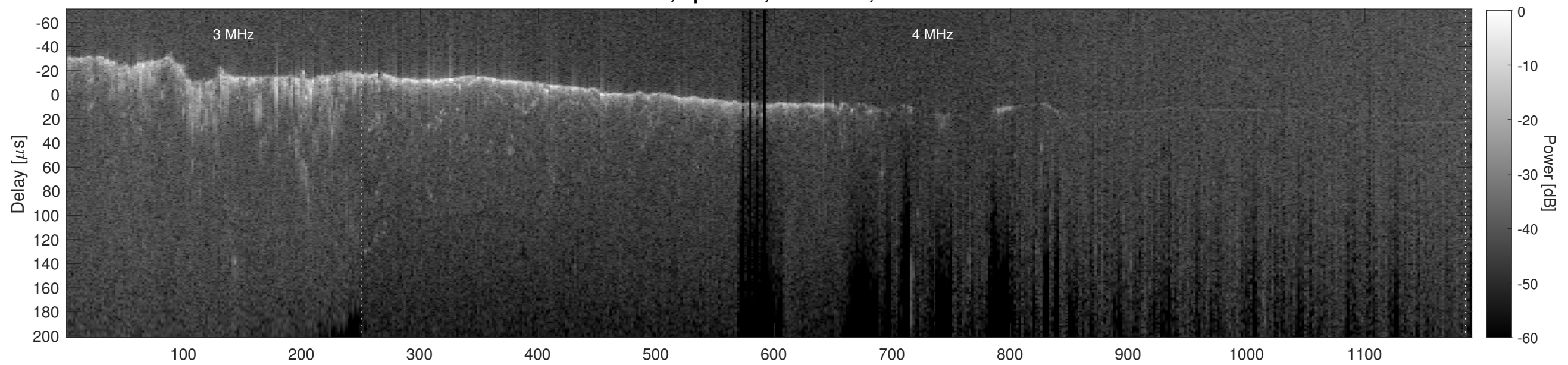
Orbit 12497, Cluttergram
