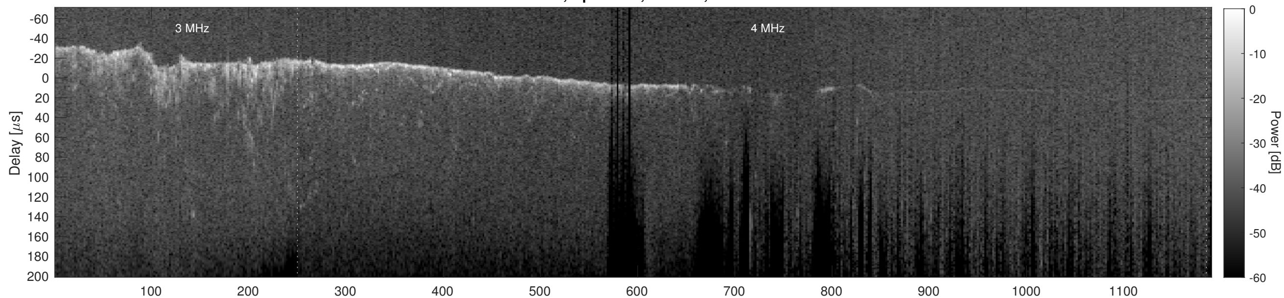
Orbit 12497, Cluttergram
