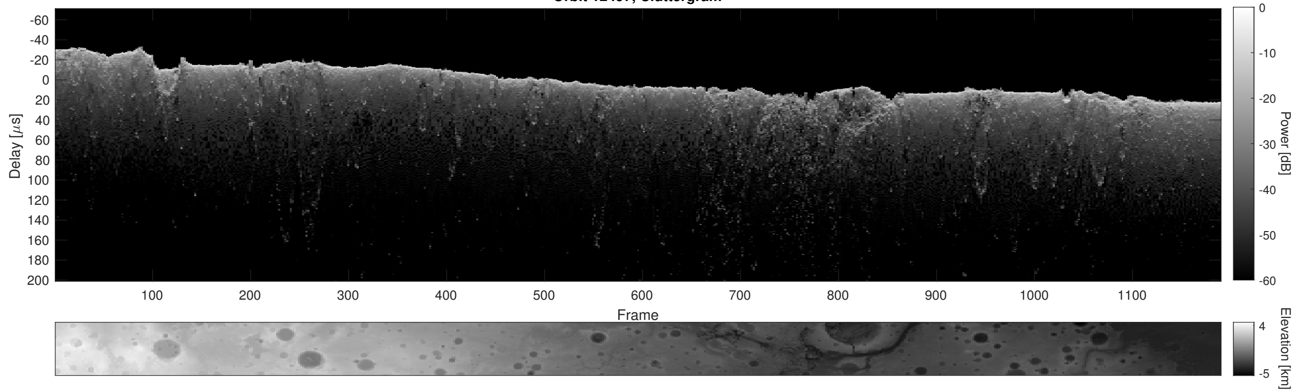
Orbit 12497, Cluttergram
