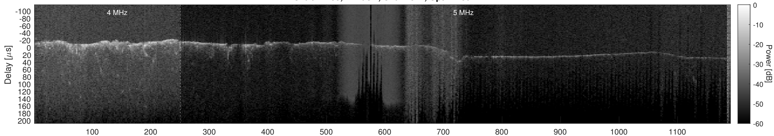
Orbit 12499, Cluttergram
