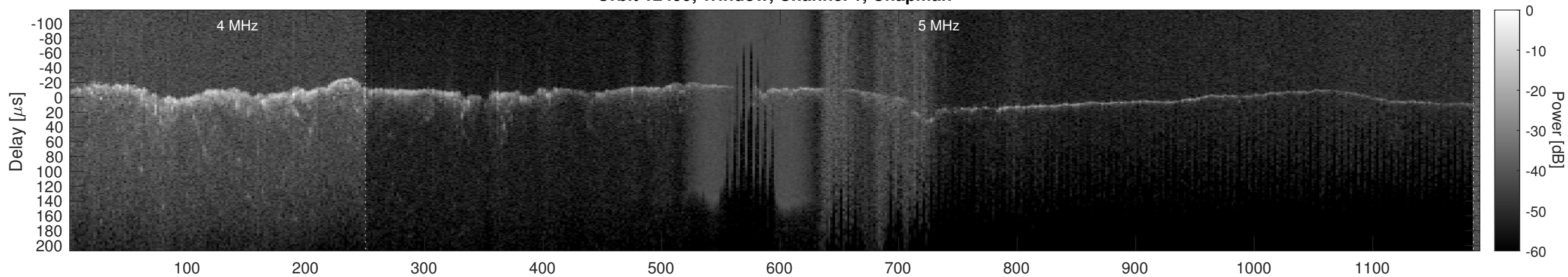
Orbit 12499, Window, Channel 1, Optimized
