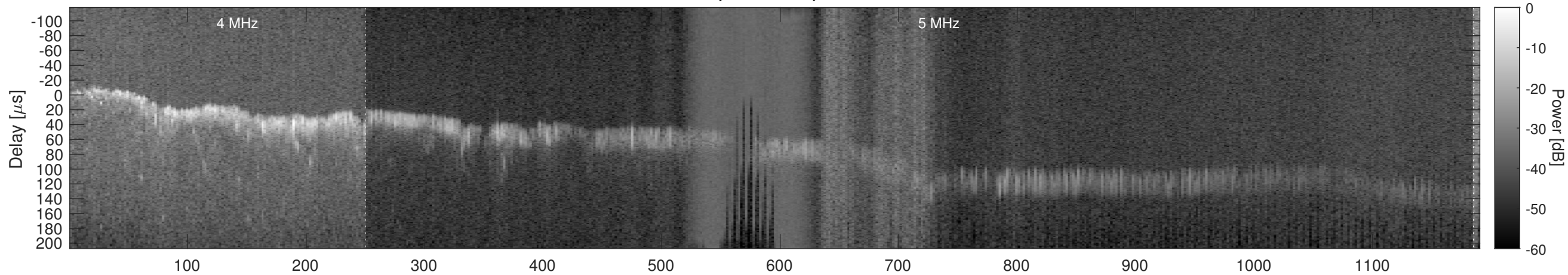
Orbit 12499, Window, Channel 1, Chapman
