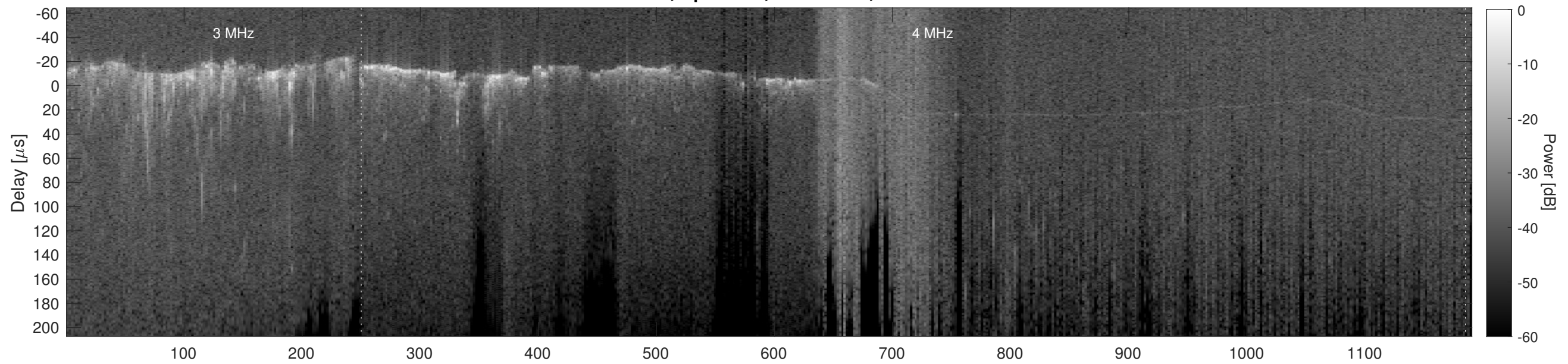
Orbit 12499, Cluttergram
