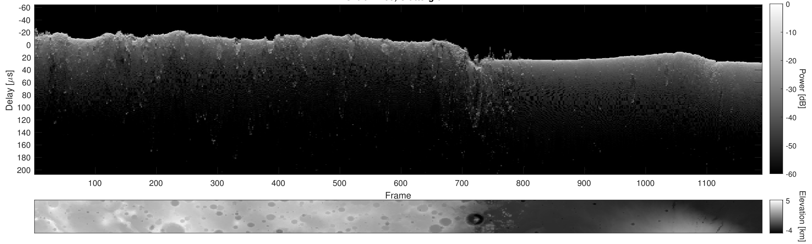
Orbit 12499, Cluttergram
