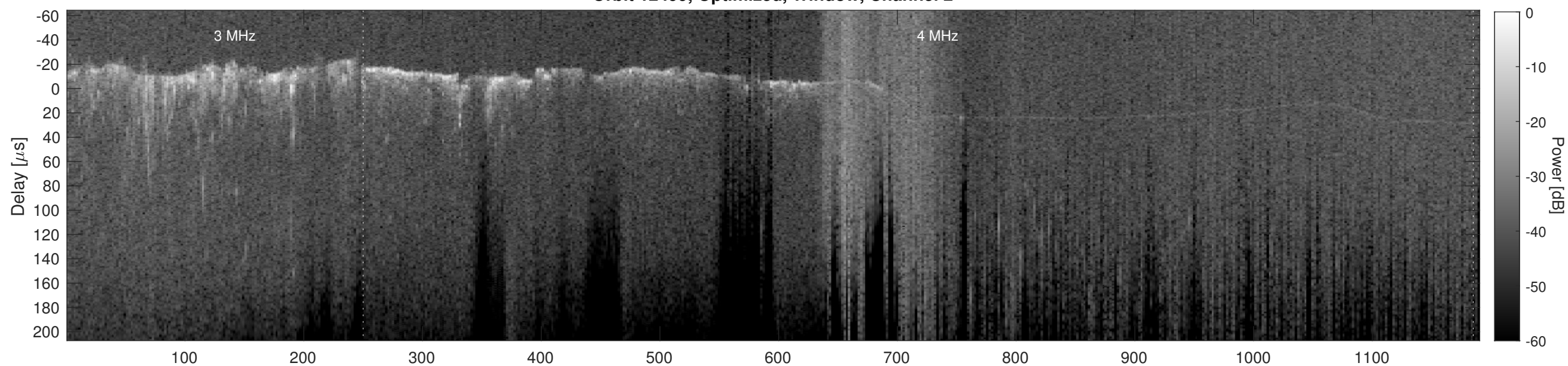
Orbit 12499, Cluttergram
