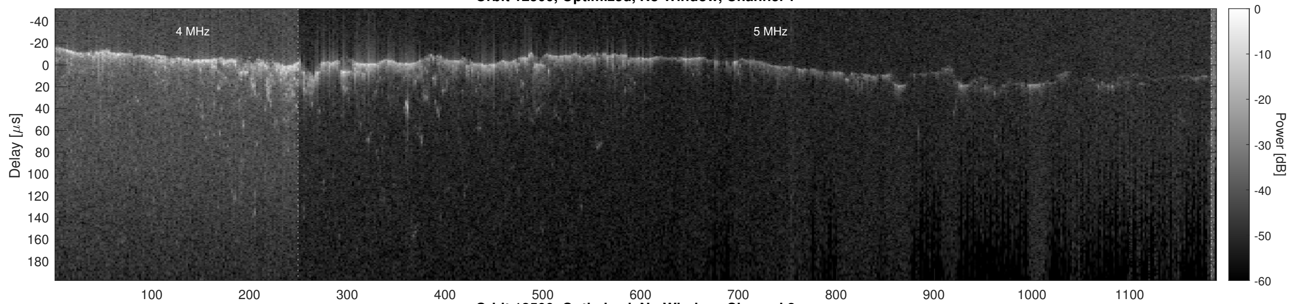
Orbit 12500, Optimized, No Window, Channel 2
